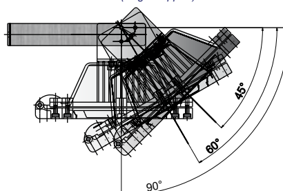
Suporte angular (AN) (Angle support)
