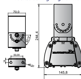
Suporte Teto Parede Angular-(TA) Bracket Ceiling Angular wall
