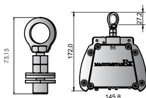
Suporte Grampo-(G□) (Clamp bracket)
