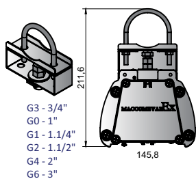
Suporte Grampo-(G□) (Clamp bracket)
